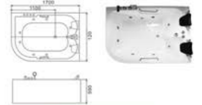
C-422(C-3085)(L) Size:1200x1700x590/mm
