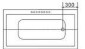
C-494-15 (R) Size: 750x1500x580/mm C-494-17 (R) Size: 800x1700x580/mm C-495 (R) Size: 1200x1700x580/mm
