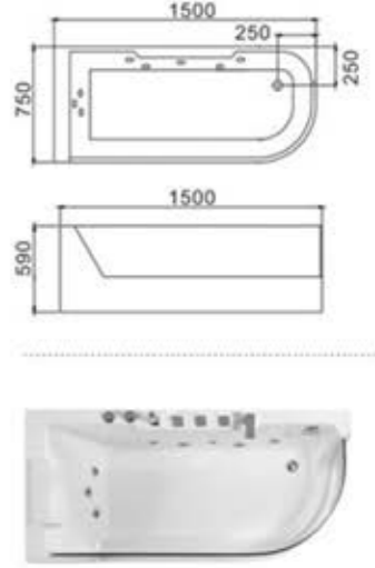
C-402(C-3132)(R) Size:750x1500x590/mm C-403(C-3133)(R) Size:800x1700x590/mm
