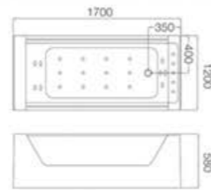
C-454 Size:1200x1700x580/mm
