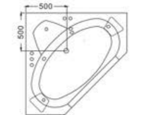
C-487-135 Size:1350x1350x580/mm C-487-150 Size:1500x1500x580/mm
