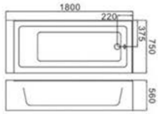
C-460(L) Size:750x1500/1600x560/mm C-461(L) Size:750x1600/1700x560/mm C-461(L) Size:750x1700/1800x560/mm
