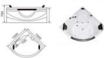
C-065 Size:1350x1350x680/mm C-066 Size:1500x1500x700/mm No.1Pillow 1号枕头 x 2
