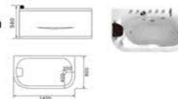
C-008 Size:800x1400x580/mm No.1Pillow 1号枕头 x 1
