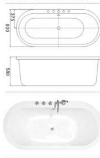
C-3211 Size:800x1700x580/mm C-3212 Size:800x1800x580/mm
