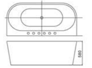
C-492-15-CL Size:750x1500x580/mm C-492-17-CL Size:800x1700x580/mm
