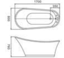
C-3150 Size:800x1700x750/mm
