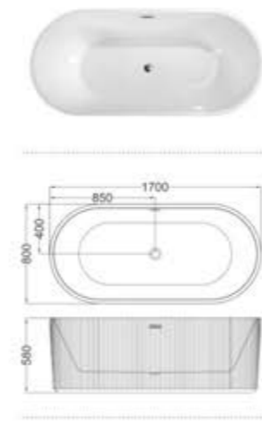
C-4269-15 Size:750x1500x580/mm C-4269-16 Size:750x1600x580/mm C-4269-17 Size:800x1700x580/mm
