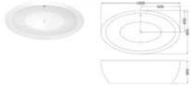
C-3262 Size:900x1850x580/mm
