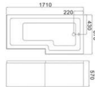
C-455(L) Size:850x1500x550/mm C-456(L) Size:850x1700x550/mm
