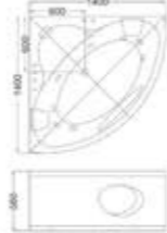
C-497-14 Size:1400x1400x580/mm C-497-15 Size:1500x1500x580/mm
