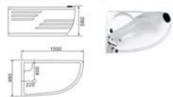
C-001 (R) Size:980x1500x580/mm No.9Pillow 9号枕头 x 1
