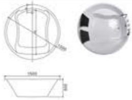
C-503 (C-3054) Size:1500x1500x500/mm
