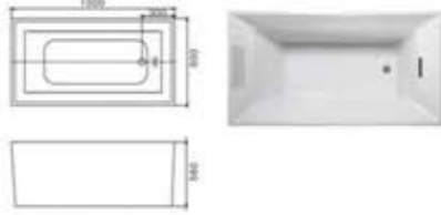
C-3100 Size:800x1500x580/mm C-3110 Size:800x1700x580/mm
