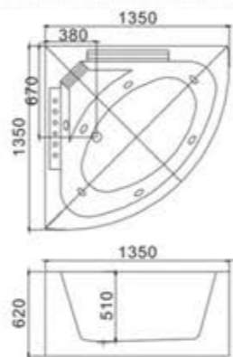
C-410(C-3066) Size:1350x1350x620/mm No.1 Pillow 13号枕头 x 1
