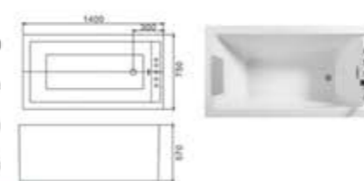
C-3123 Size:750x1400x570/mm C-3124 Size:750x1500x570/mm C-3125 Size:750x1600x570/mm C-3126 Size:750x1700x570/mm
