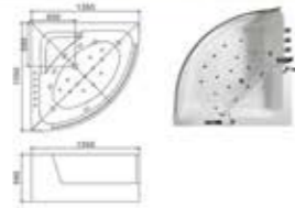
C-400(C-3130) Size:1350x1350x590/mm C-401(C-3131) Size:1500x1500x590/mm
