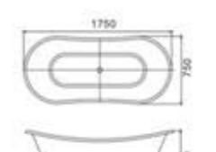
C-3140 Size:750x1750x780/mm Size:29.5x68.9x30.7/mm
