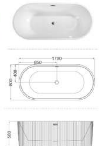
C-4269-BL-15 Size:750x1500x580/mm C-4269-BL-16 Size:750x1600x580/mm C-4269-BL-17 Size:800x1700x580/mm
