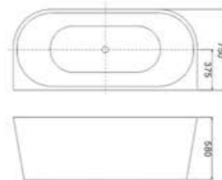
C-3218 Size:750x1300x580/mm C-3219 Size:750x1400x580/mm C-3220 Size:750x1500x580/mm C-3221 Size:750x1700x580/mm
