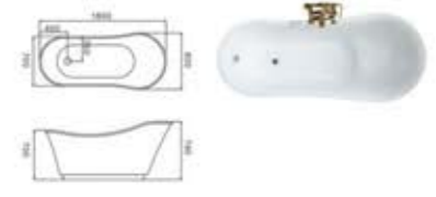
C-3003-1 Size:830x1800x780/mm
