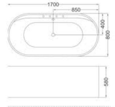
C-3229-HLT Size:800x1700x580/mm
