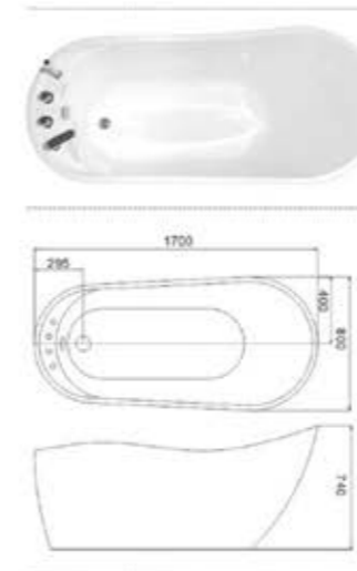
C-3214 Size:800x1700x740/mm
