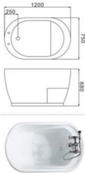
C-404 (C-3016) Size:750x1200x680/mm
