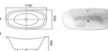
C-3138 Size:800x1700x680/mm Size:31.4x66.9x26.8/mm C-3139 Size:800x1800x700/mm Size:31.4x70.8x27.5/mm
