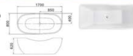
C-3236 Size:800x1700x620/mm
