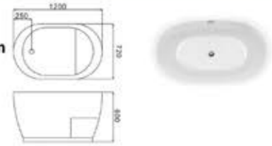
C-3250 Size:720x1200x600/mm
