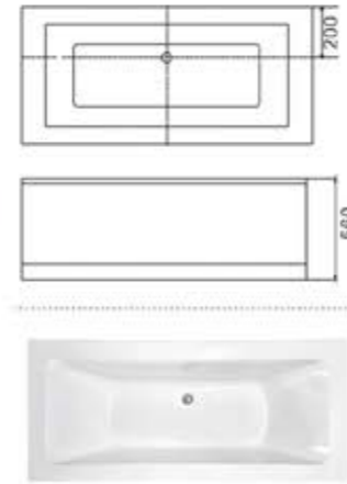
C-076-70 (L) Size:700x1700x560/mm C-076-75 (L) Size:750x1700x560/mm C-076-75 (L) Size:810x1700x560/mm
