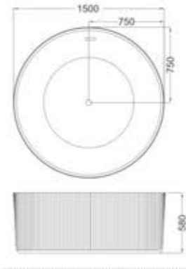
C-4270-135 Size:1350x1350x580/mm C-4270-150 Size:1500x1500x580/mm
