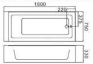
C-457(L) Size:750x1500/1600x300/mm C-458(L) Size:750x1600/1700x300/mm C-459(L) Size:750x1700/1800x330/mm
