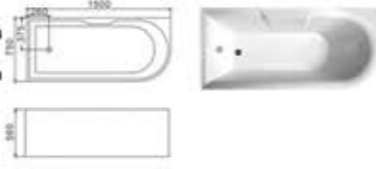
C-3115(R) Size:750x1500x560/mm C-3022(R) Size:750x1700x560/mm
