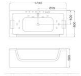
SH-110-15 Size:800x1500x580/mm SH-110-16 Size:800x1600x580/mm SH-110-17 Size:800x1700x580/mm
