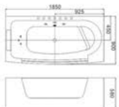
C-468 Size:900x1850x580/mm
