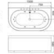
C-466 Size:800x1500x580/mm C-467 Size:800x1700x580/mm
