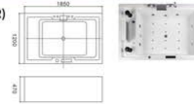
C-500-TV(C-3142-TV)(R) Size:1200x1850x470/mm
