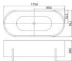
C-3226 Size:750x1700x550/mm
