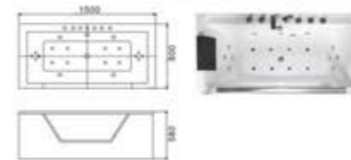
C-426(C-3089) Size:800x1500x580/mm C-427(C-3090) Size:800x1600x580/mm C-428(C-3091) Size:800x1700x580/mm C-429(C-3092) Size:800x1800x580/mm No.14 Pillow 14号枕头 x 1
