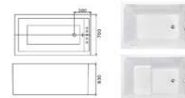
C-3260-10 Size:700x1000x630/mm C-3260-11 Size:700x1100x630/mm C-3260-12 Size:700x1200x630/mm C-3260-13 Size:700x1300x630/mm
