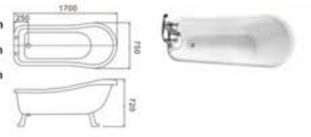
C-3136-2 Size:750x1500x700/mm C-3179 Size:750x1600x710/mm C-3137-2 Size:750x1700x720/mm
