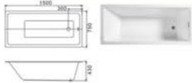
C-522(C-3134-X) Size:750x1500x430/mm C-523(C-3135-X) Size:750x1700x430/mm
