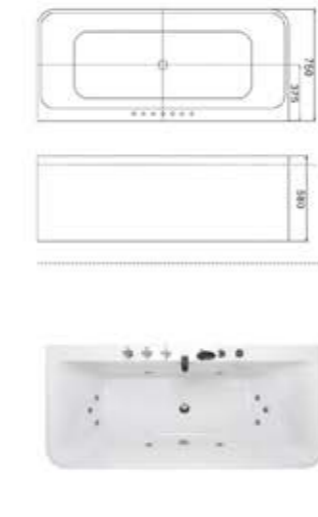
C-3246-15 Size:750x1500x580/mm C-3246-16 Size:750x1600x580/mm C-3246-17 Size:750x1700x580/mm C-3246-18 Size:800x1800x580/mm
