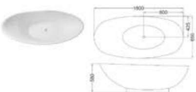
C-3031 Size:850x1800x580/mm C-3036 Size:780x1500x570/mm
