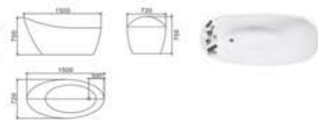
C-3113 Size:720x1500x700/mm C-3114 Size:750x1700x730/mm
