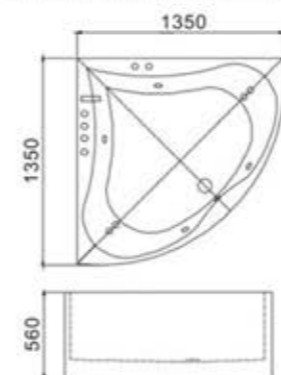
C-413(C-3069) Size:1350x1350x560/mm
