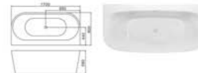
C-3243 Size:800x1700x580/mm
