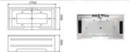
C-430(C-3093) Size:800x1500x590/mm C-431(C-3094) Size:800x1600x590/mm C-432(C-3095) Size:800x1700x590/mm No.17 Pillow 17号枕头 x 2
