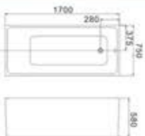
C-3169 Size:750x1400x580/mm C-3170 Size:750x1500x580/mm C-3171 Size:750x1600x580/mm C-3172 Size:750x1700x580/mm
