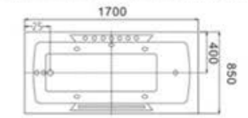
C-441 (C-3062-1) (R) Size:850x1500x620/mm C-442 (C-3063-1) (R) Size:850x1600x620/mm C-442 (C-3064-1) (R) Size:850x1700x620/mm No.1Pillow 15号枕头 x 1
