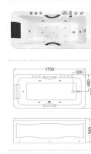
SH-104-15-L Size:800x1500x580/mm SH-104-16-L Size:800x1600x580/mm SH-104-17-L Size:800x1700x580/mm
