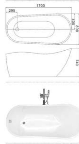
C-3213 Size:800x1700x740/mm
