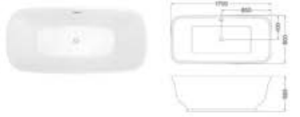
C-3263-15 Size:720x1500x580/mm C-3263-16 Size:800x1700x580/mm
