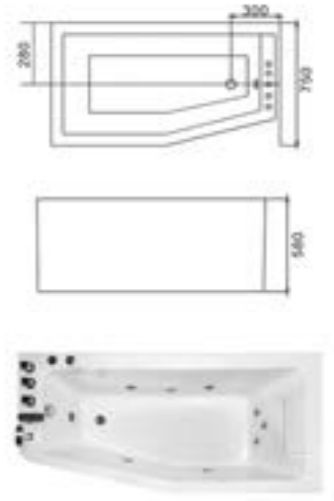
C-483-17(L) Size:800x1700x580/mm
