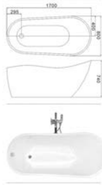
C-3213 Size:800x1700x740/mm
