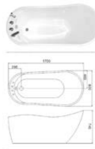
C-3214 Size:800x1700x740/mm
