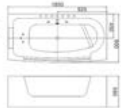
C-468 Size:900x1850x580/mm
