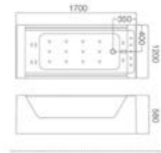
C-454 Size:1200x1700x580/mm
