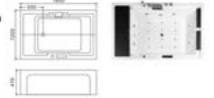
C-500-(C-3142)(R) Size:1200x1850x470/mm
