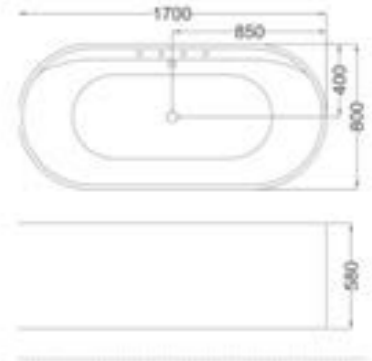
C-3229-HLT Size:800x1700x580/mm
